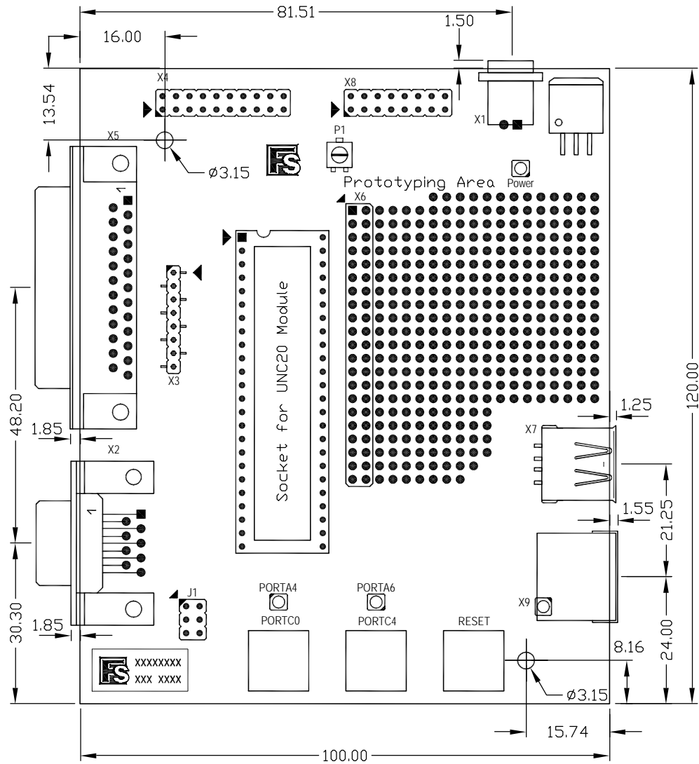
TOP View
