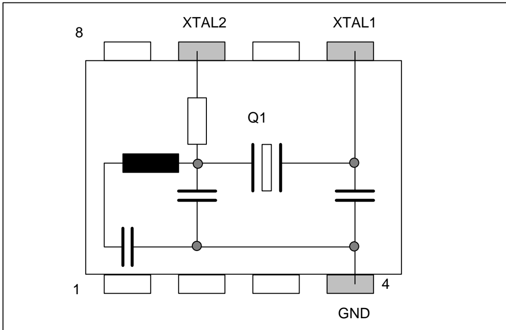
Figure 9: External crystal
