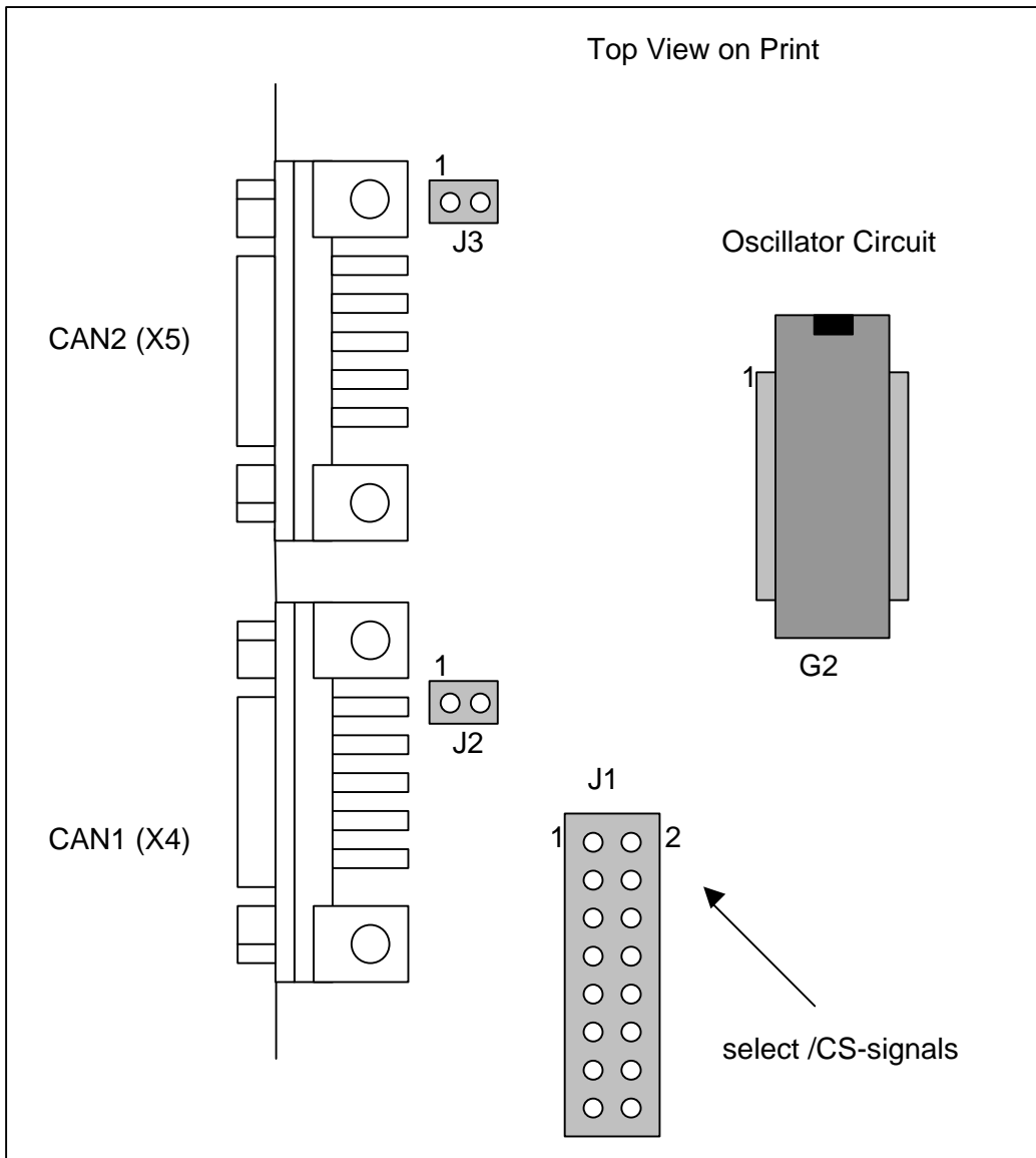
Figure 3: Selection of Chip Select
