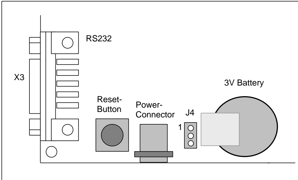
Figure 8: Power Supply
