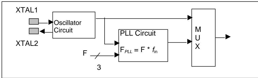
Figure 5: Clock generation
