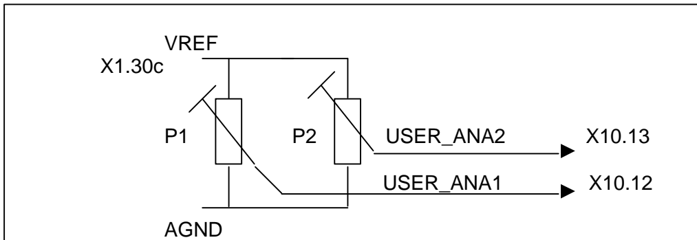
Figure 7: Potentiometer (P1, P2)
