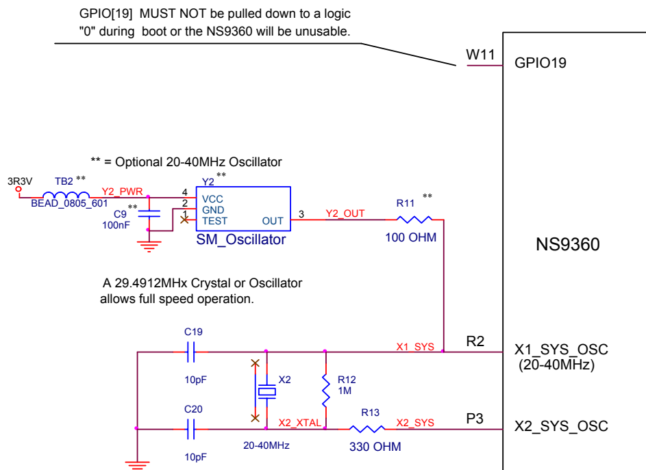
Figure 3: NS9360 system clock
