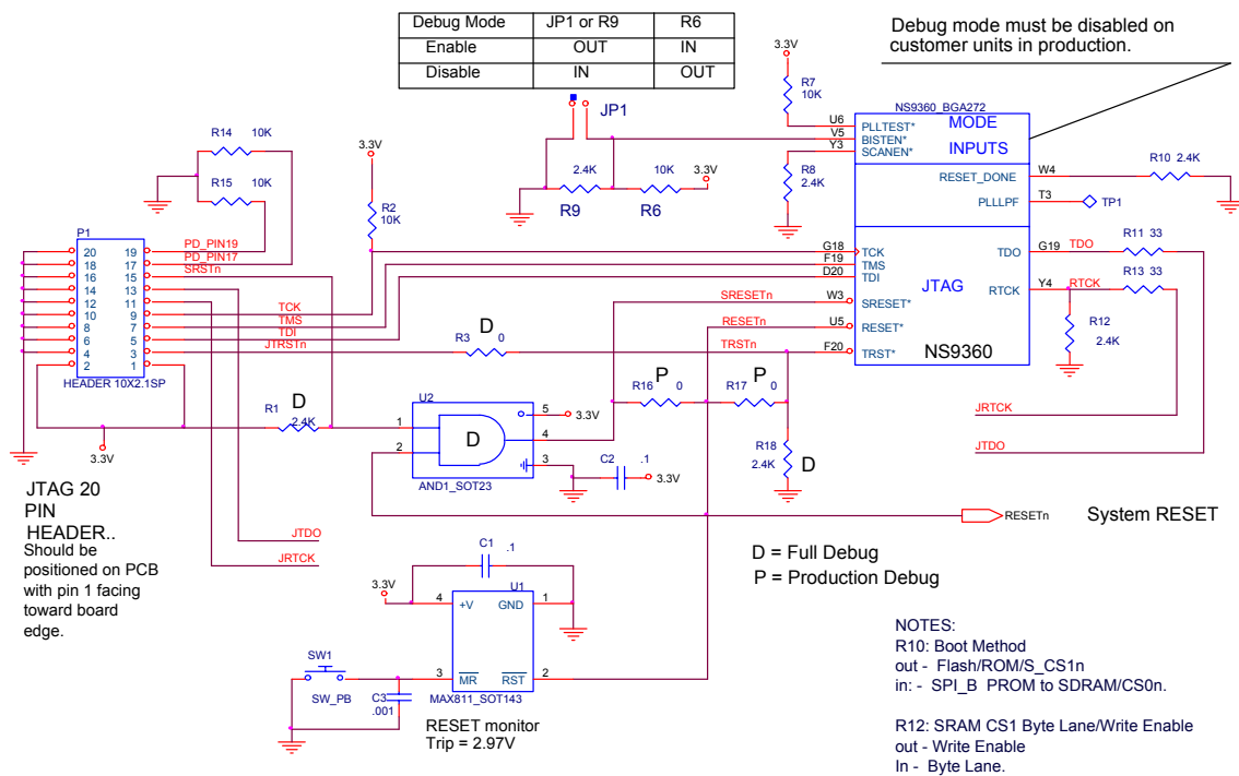
Figure 6: JTAG interface
