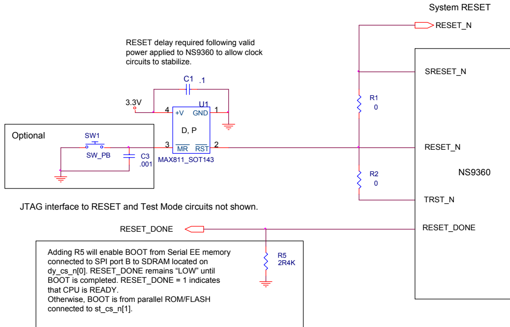
Figure 2: Sample reset circuit
