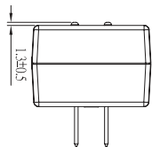
Digi XBee-PRO Range Extender - Top (North America unit only)
