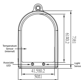
Digi XBee-PRO Range Extender - Front
