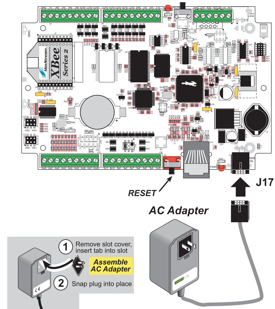
Figure 2. Power Supply Connections
