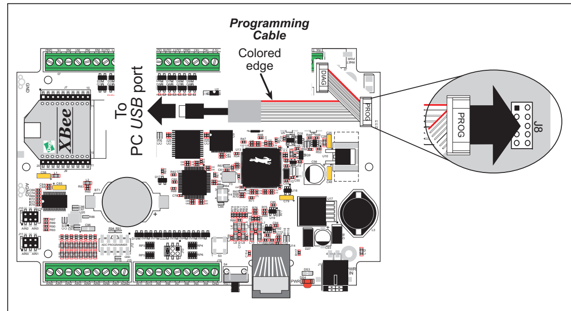
Figure 1. Connect Programming Cable and Power Supply
