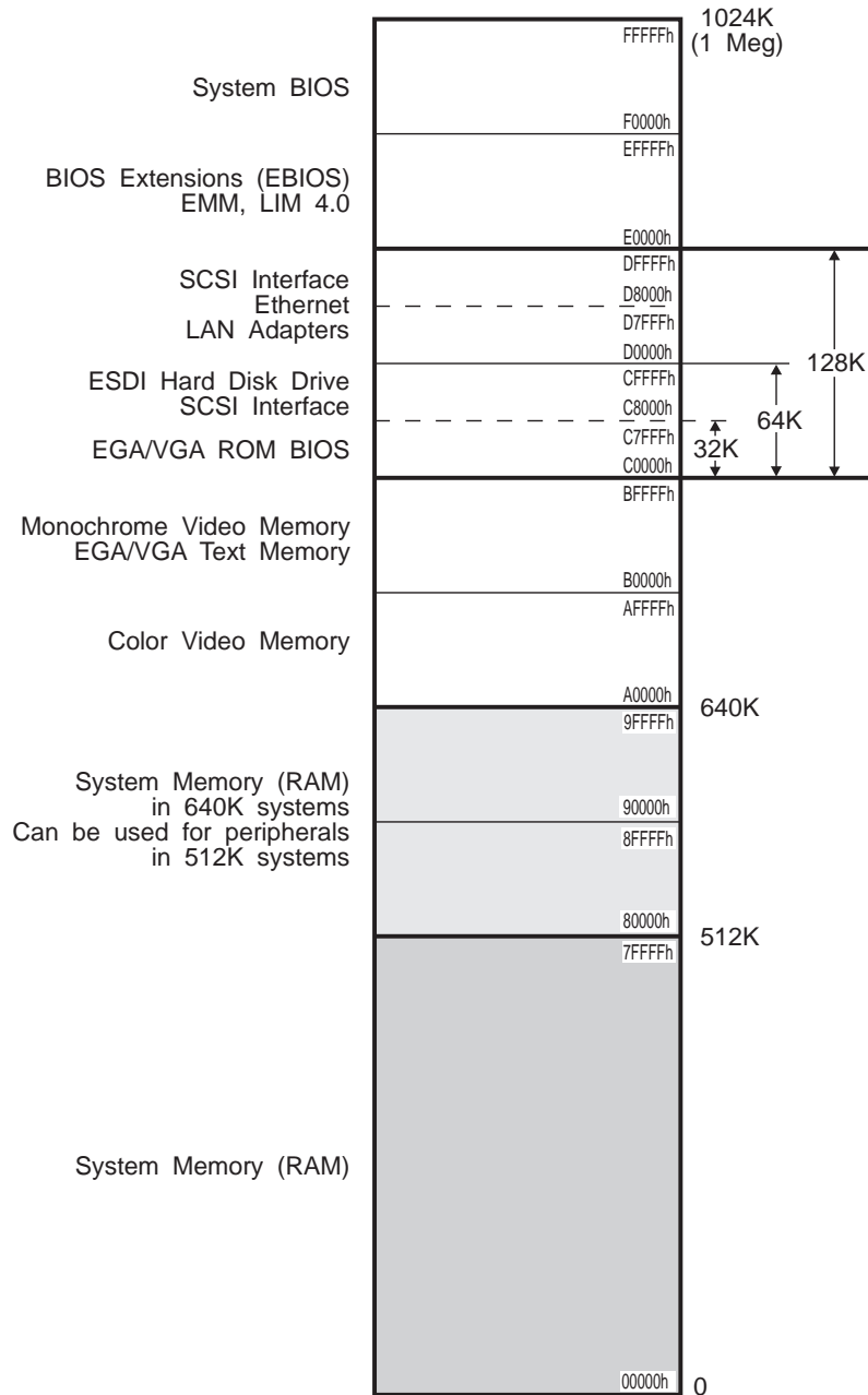
Figure 7 Typical PC Memory Usage - 1st Megabyte
