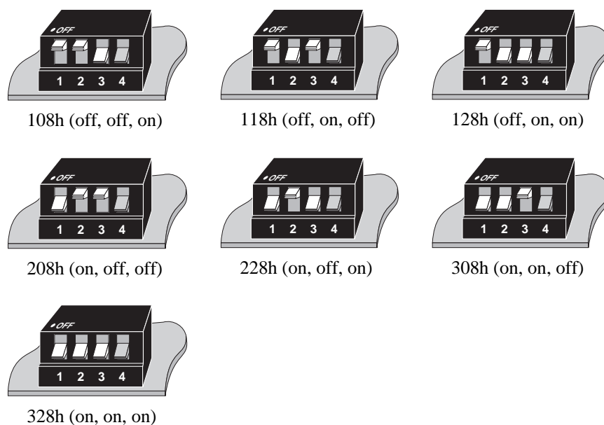
Figure 3 DIP Switch Settings for I/O Port Starting Address
