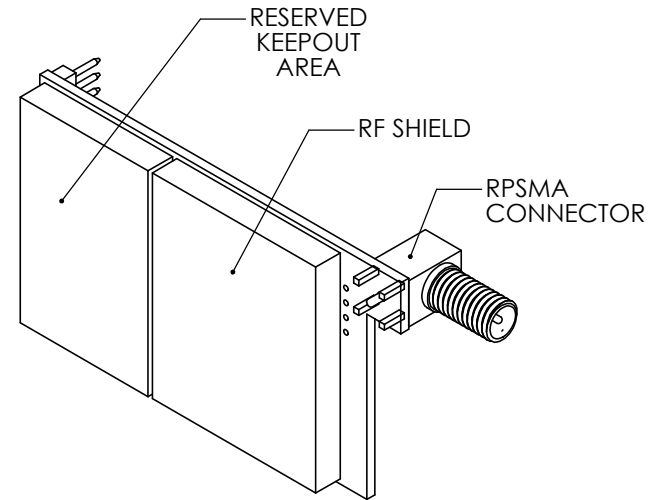
ISOMETRIC VIEW
