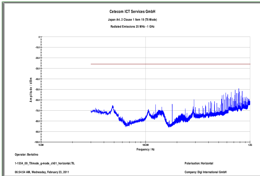
Plot 3: TX mode, lowest channel, up to 1 GHz, horizontal
