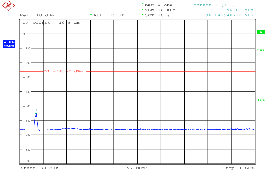
Plot 1: TX mode, lowest channel, 30 MHz to 1 GHz
