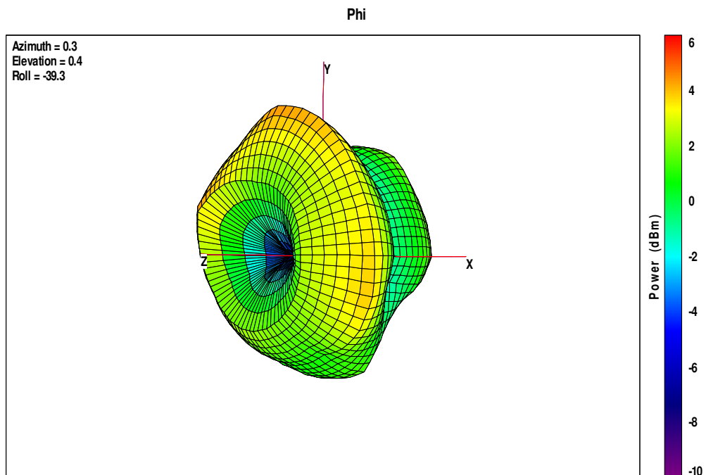
Plot 8: Antenna diagram highest channel (horizontal) – all values are in dBm
