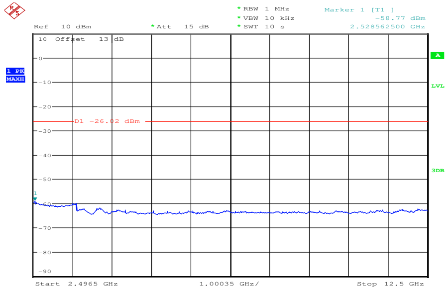
Plot 5: TX mode, lowest channel, 2496.5 MHz to 12500 MHz
