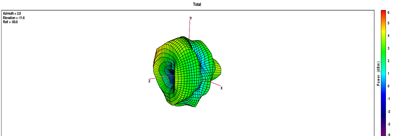
Plot 6: Antenna diagram middle channel (vertical & horizontal – vectorial summation) – all values are in dBm
