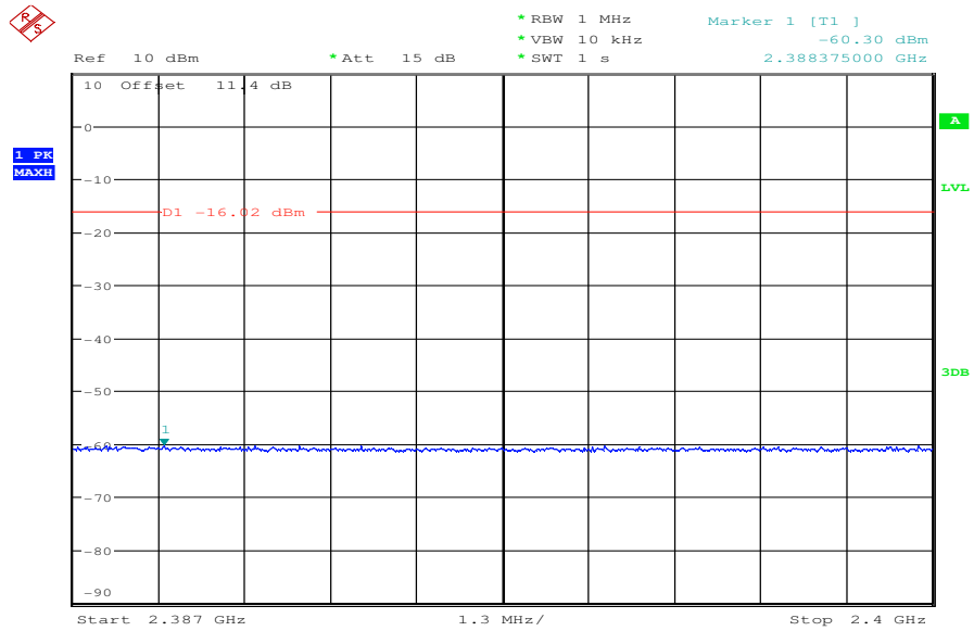
Plot 13: TX mode, highest channel, 2387 MHz to 2400 MHz
