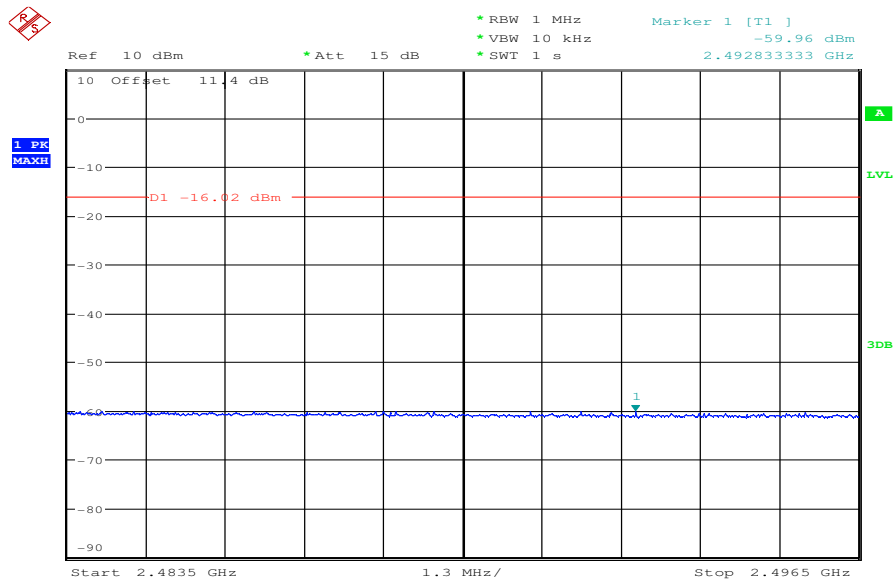
Plot 9: TX mode, middle channel, 2483.5 MHz to 2496.5 MHz
