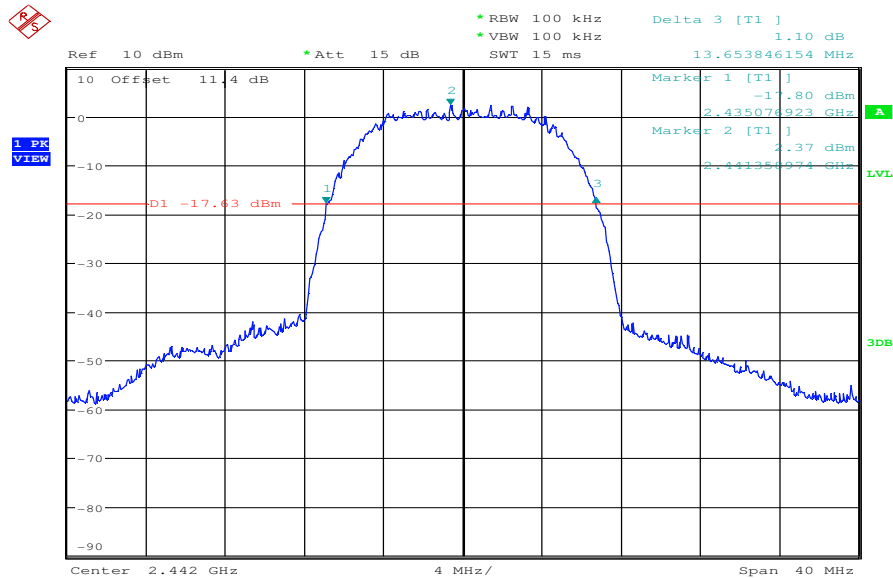
Plot 4: middle channel, 20 dB bandwidth
