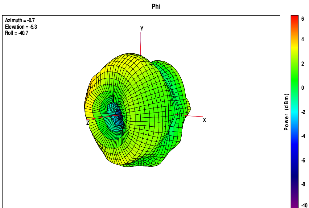
Plot 5: Antenna diagram middle channel (horizontal) – all values are in dBm
