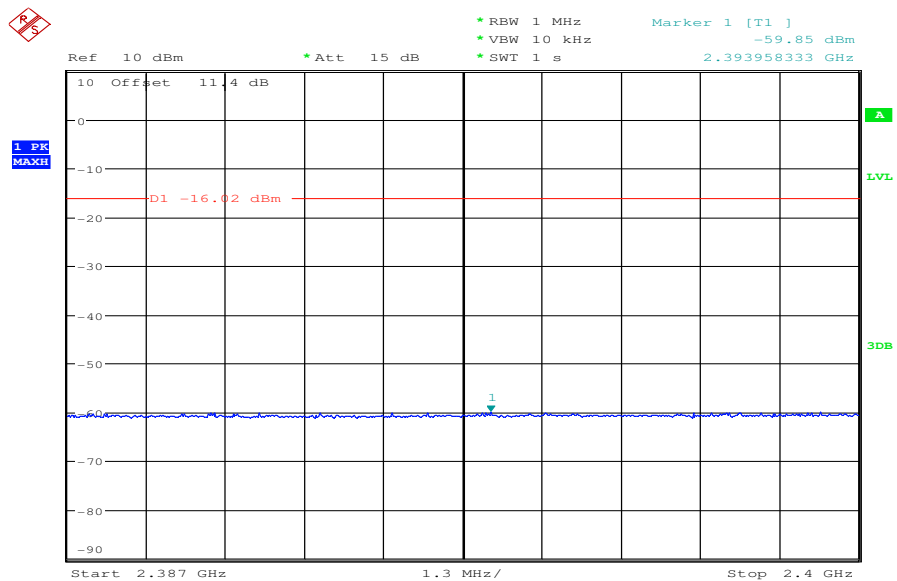
Plot 8: TX mode, middle channel, 2387 MHz to 2400 MHz
