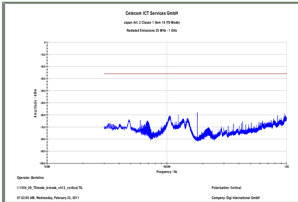
Plot 9: TX mode, highest channel, up to 1 GHz, vertical
