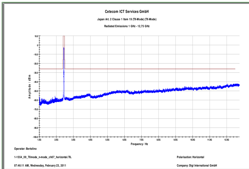
Plot 8: TX mode, middle channel, 1 GHz to 12.75 GHz, horizontal
