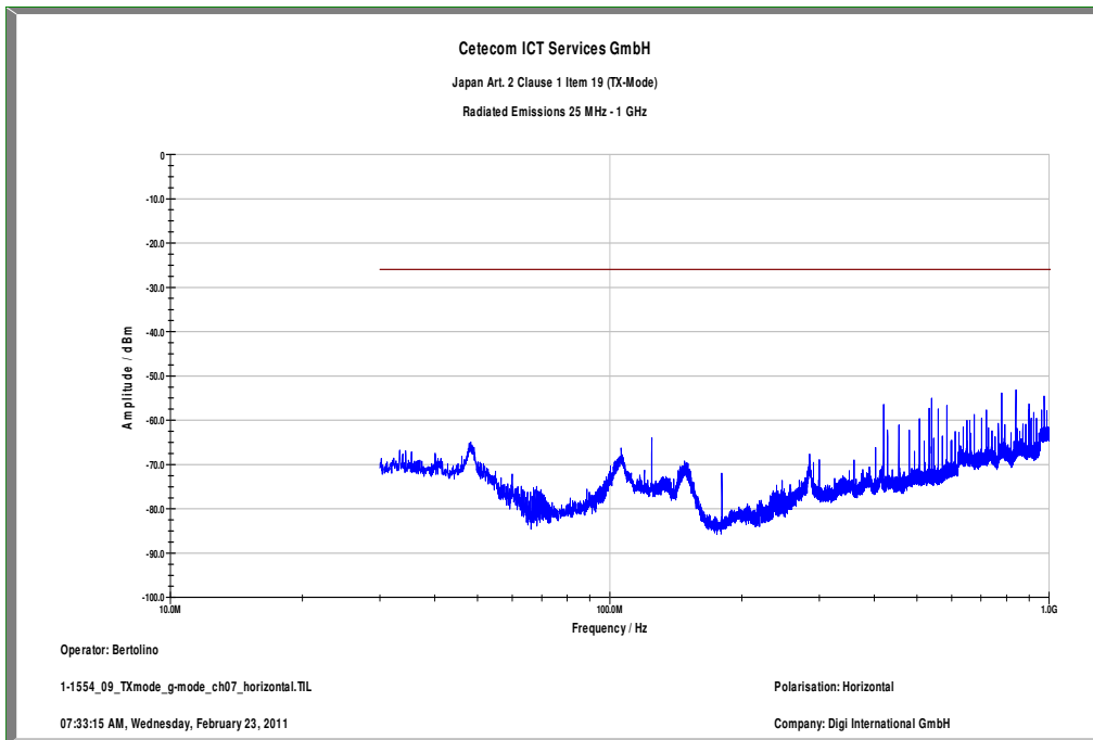
Plot 7: TX mode, middle channel, up to 1 GHz, horizontal
