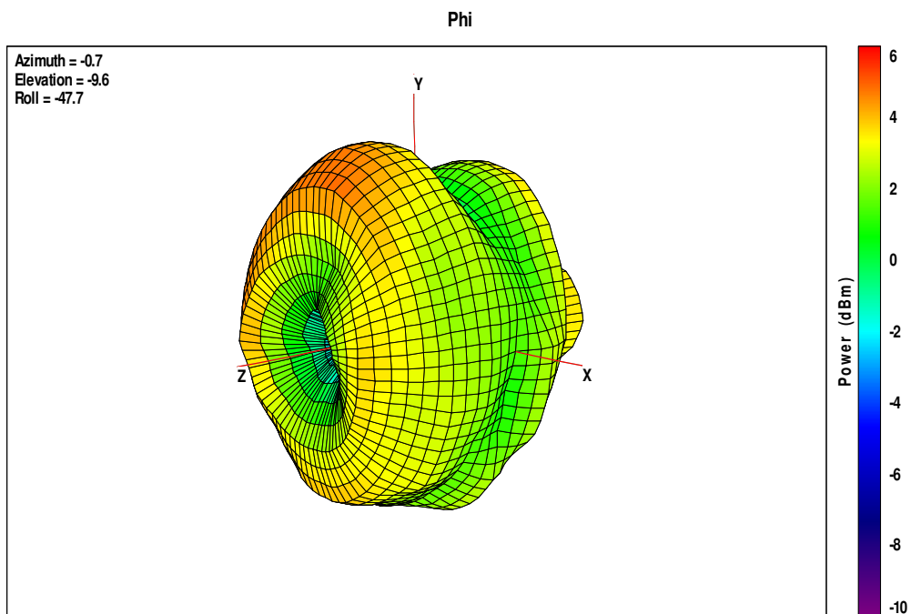
Plot 2: Antenna diagram lowest channel (horizontal) – all values are in dBm
