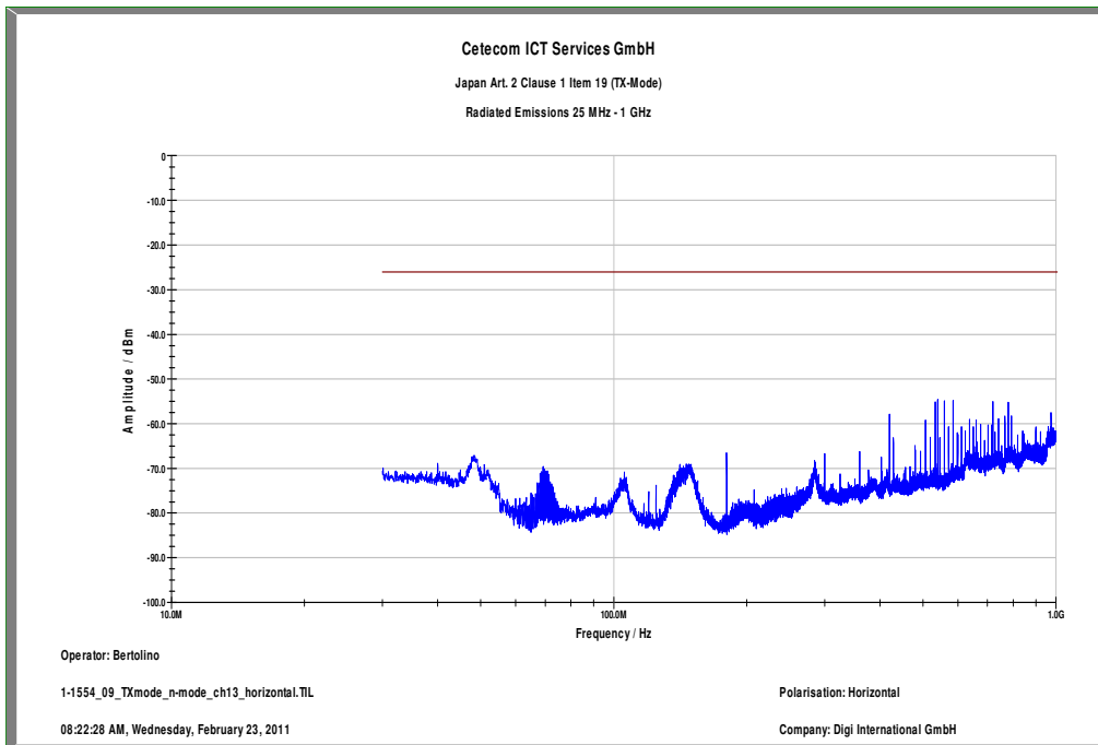
Plot 11: TX mode, highest channel, up to 1 GHz, horizontal
