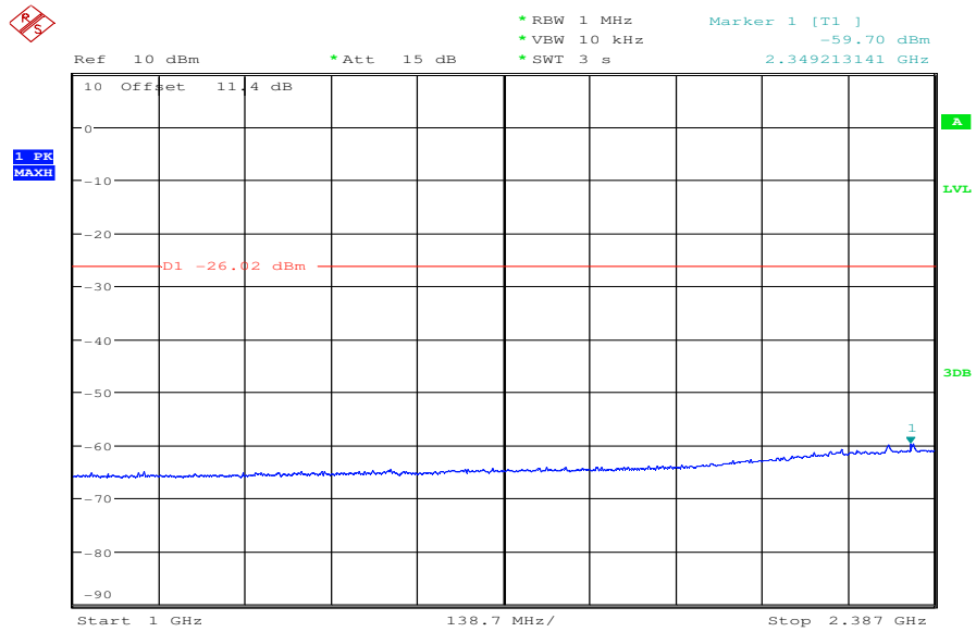
Plot 12: TX mode, highest channel, 1 GHz to 2387 MHz
