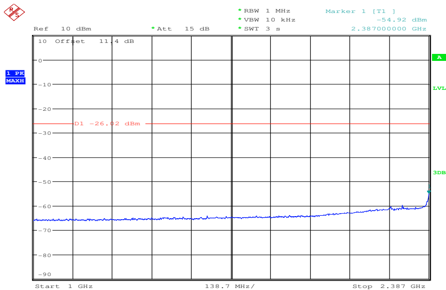
Plot 2: TX mode, lowest channel, 1 GHz to 2387 MHz
