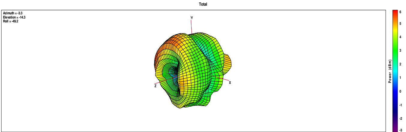
Plot 3: Antenna diagram lowest channel (vertical & horizontal – vectorial summation) – all values are in dBm
