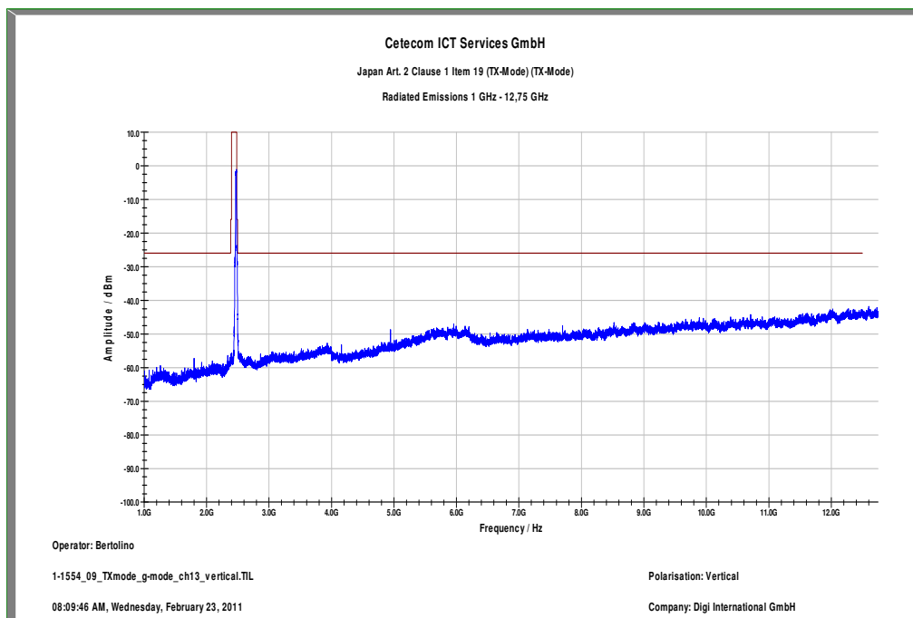
Plot 10: TX mode, highest channel, 1 GHz to 12.75 GHz, vertical
