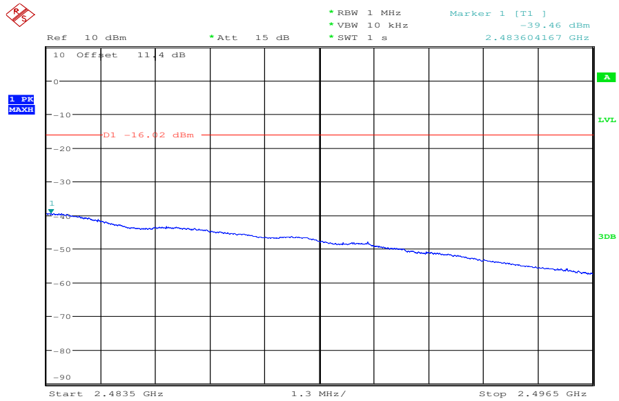
Plot 14: TX mode, highest channel, 2483.5 MHz to 2496.5 MHz
