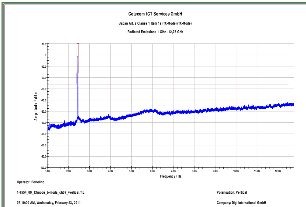
Plot 6: TX mode, middle channel, 1 GHz to 12.75 GHz, vertical
