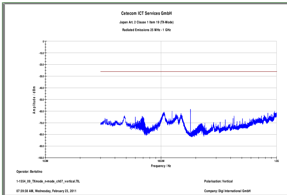
Plot 5: TX mode, middle channel, up to 1 GHz, vertical
