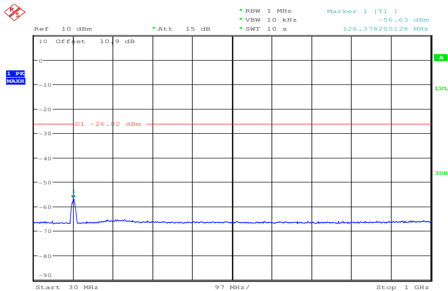
Plot 6: TX mode, middle channel, 30 MHz to 1 GHz
