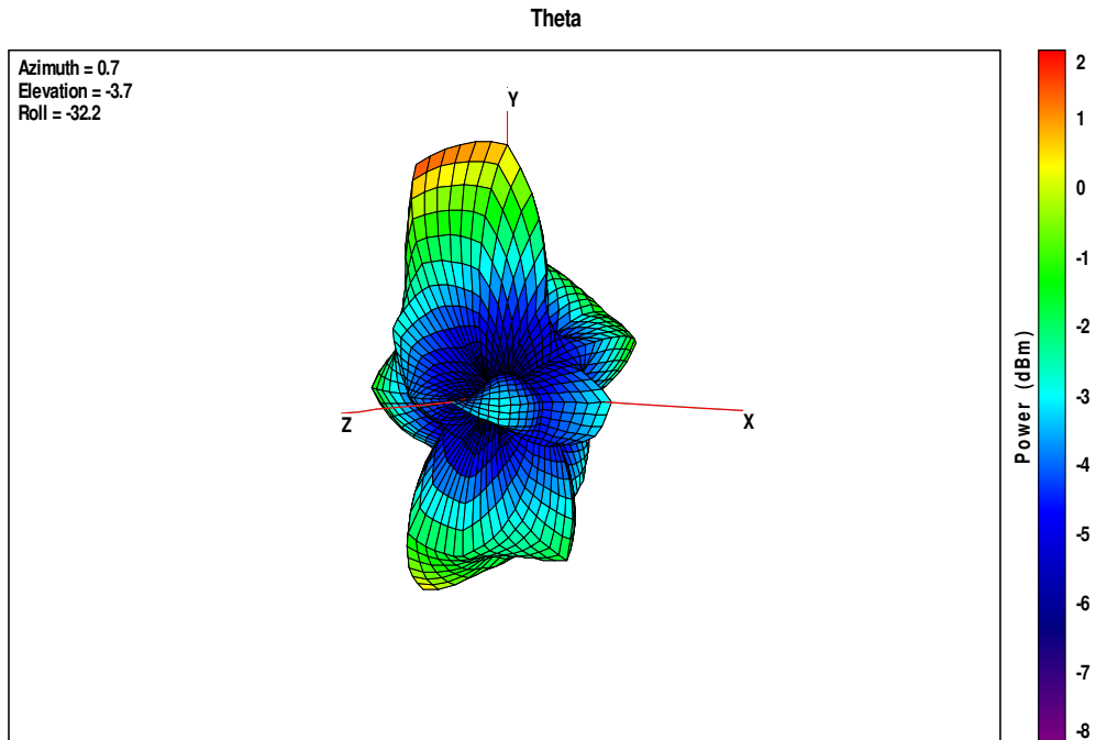
Plot 7: Antenna diagram highest channel (vertical) – all values are in dBm
