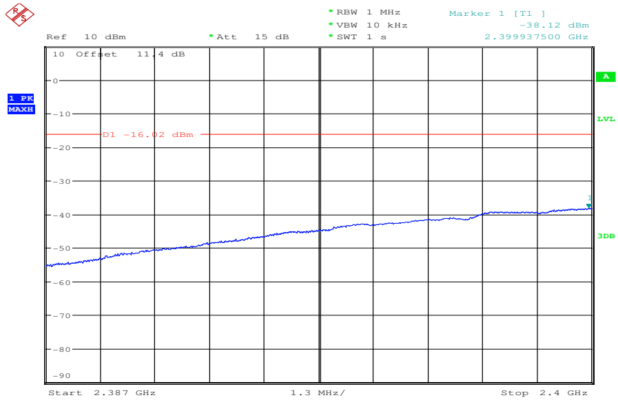
Plot 3: TX mode, lowest channel, 2387 MHz to 2400 MHz
