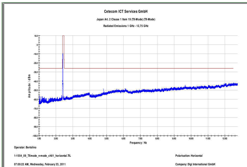
Plot 4: TX mode, lowest channel, 1 GHz to 12.75 GHz, horizontal
