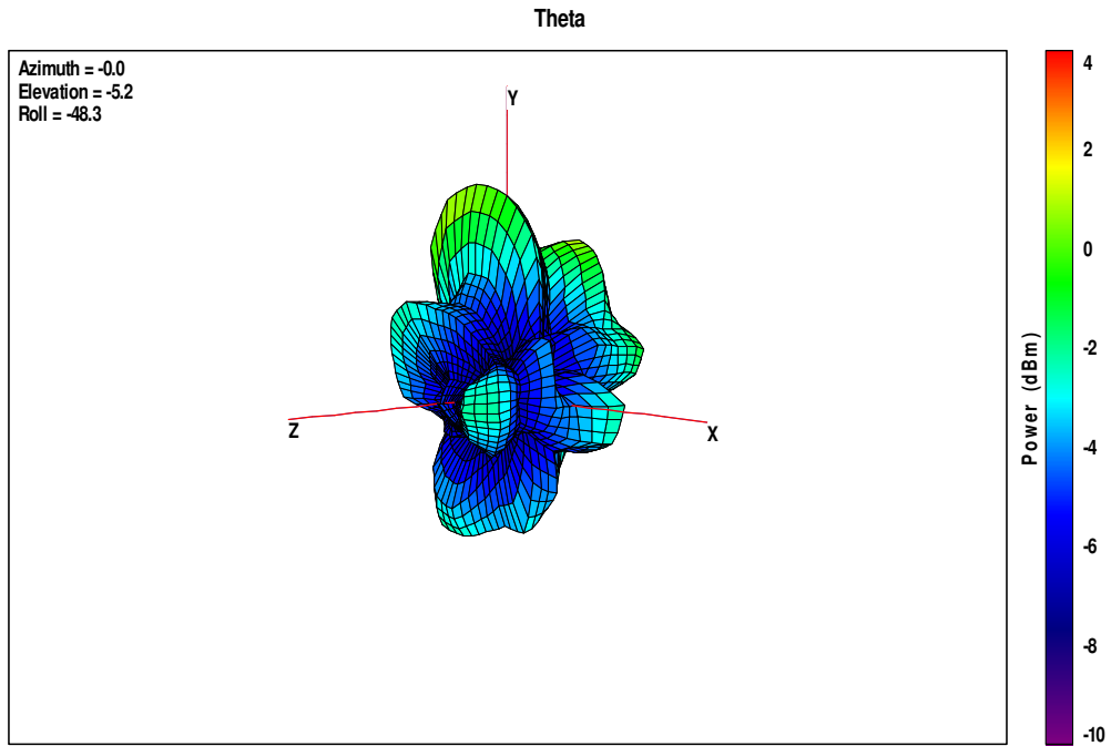
Plot 4: Antenna diagram middle channel (vertical) – all values are in dBm
