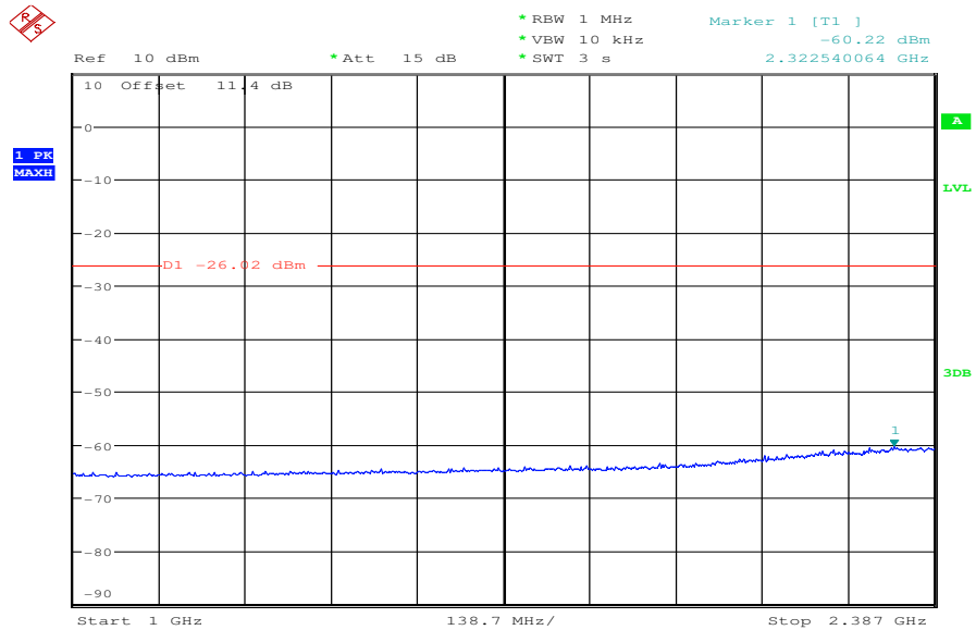
Plot 7: TX mode, middle channel, 1 GHz to 2387 MHz
