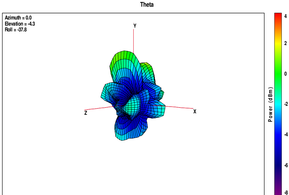
Plot 1: Antenna diagram lowest channel (vertical) – all values are in dBm
