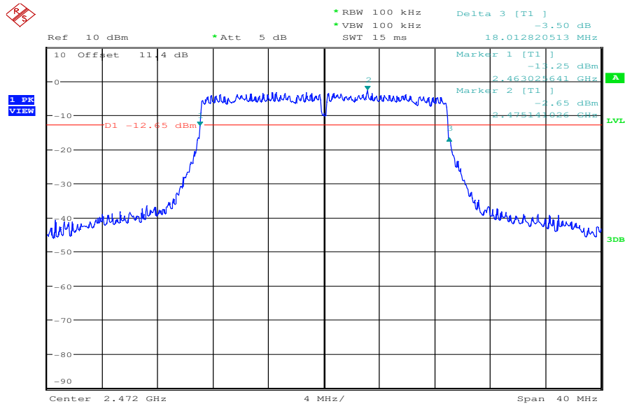
Plot 5: highest channel, 10 dB bandwidth
