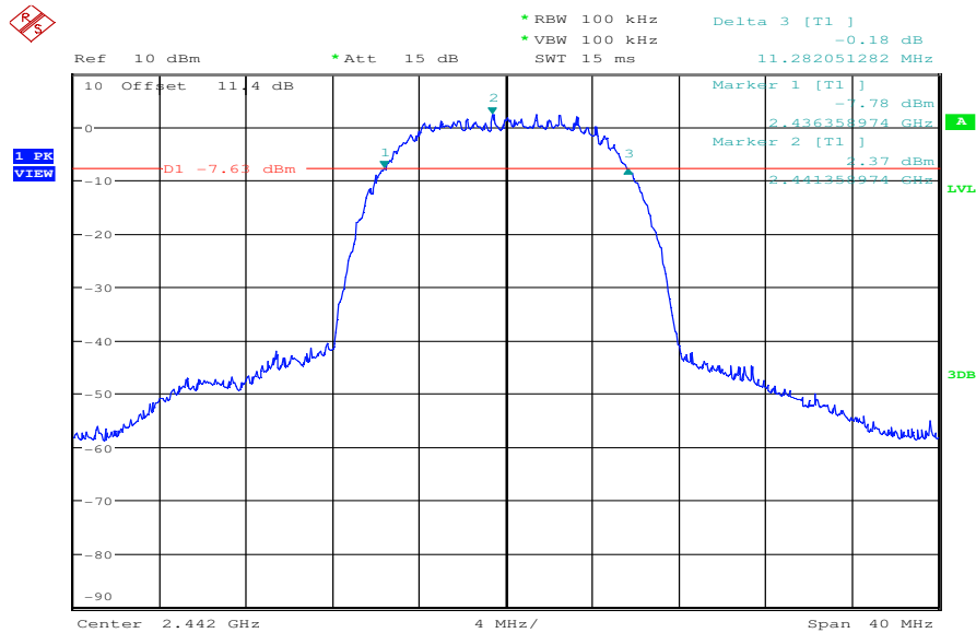
Plot 3: middle channel, 10 dB bandwidth
