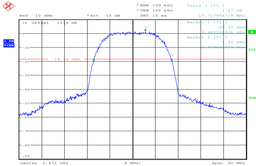
Plot 6: highest channel, 20 dB bandwidth
