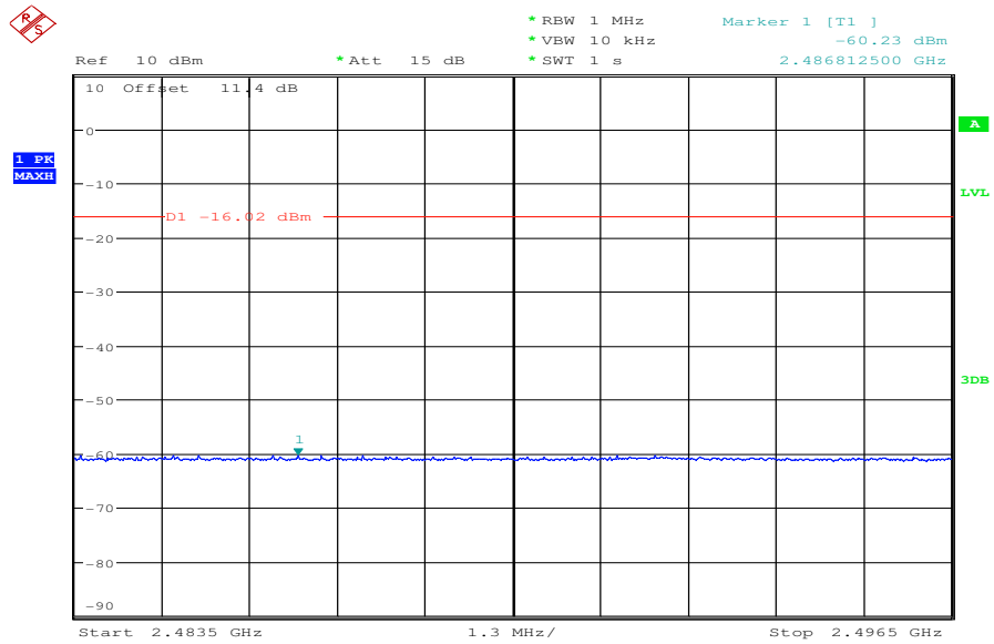
Plot 4: TX mode, lowest channel, 2483.5 MHz to 2496.5 MHz
