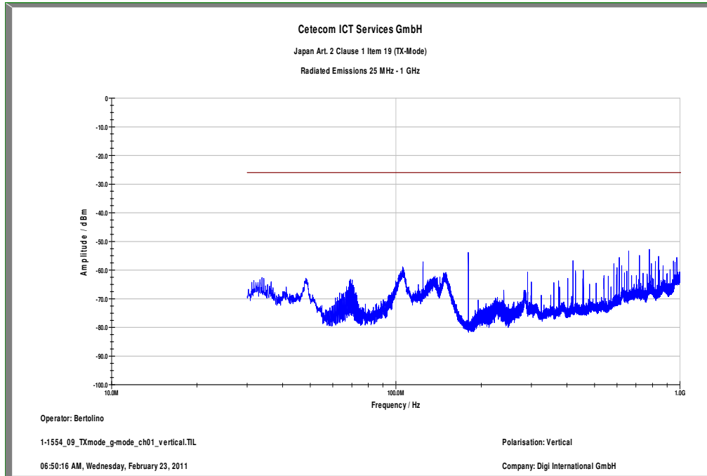
Plot 1: TX mode, lowest channel, up to 1 GHz, vertical
