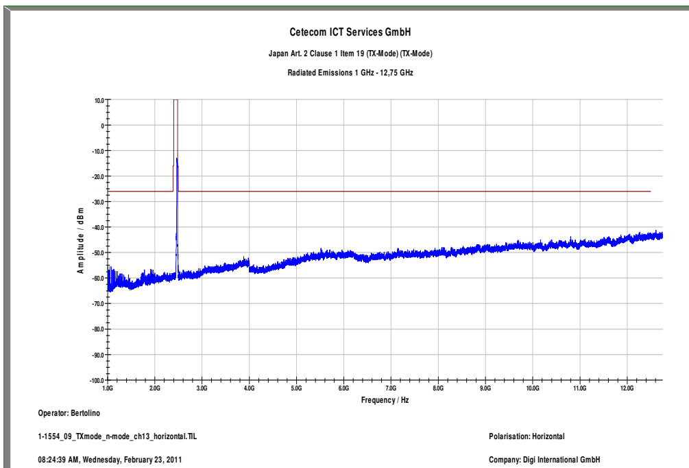
Plot 12: TX mode, highest channel, 1 GHz to 12.75 GHz, horizontal
