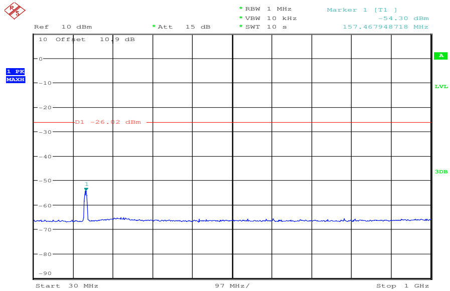
Plot 11: TX mode, highest channel, 30 MHz to 1 GHz
