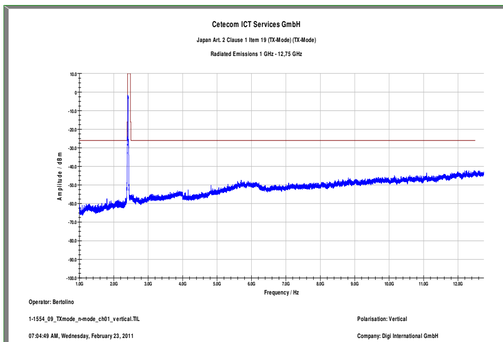
Plot 2: TX mode, lowest channel, 1 GHz to 12.75 GHz, vertical
