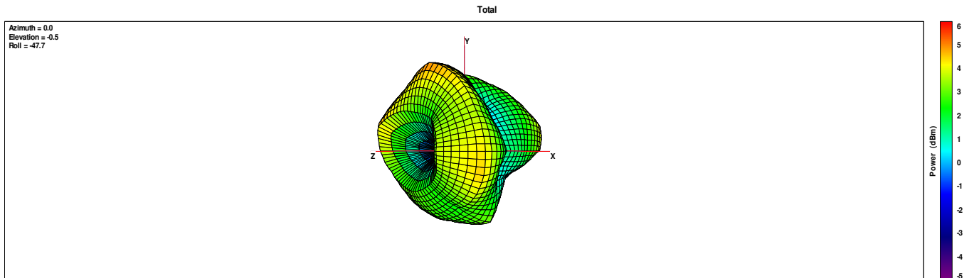
Plot 9: Antenna diagram highest channel (vertical & horizontal – vectorial summation) – all values are in dBm
