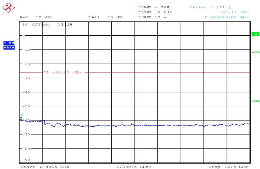
Plot 10: TX mode, middle channel, 2496.5 MHz to 12500 MHz
