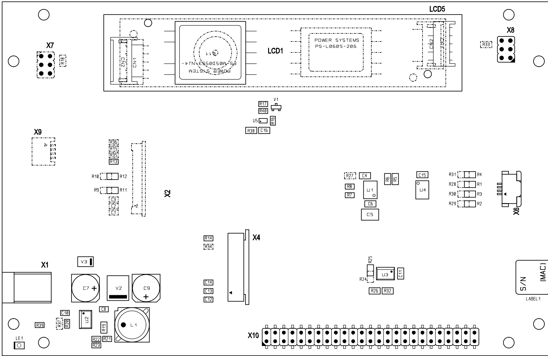
LCDAPKITJS_0 Placement TOP 27.09.06
